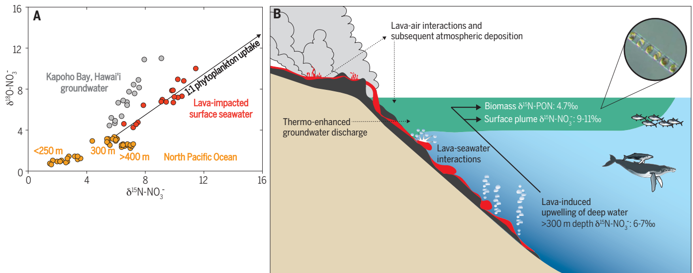
Fig. 4. Nitrate origins. (A) \delta^{15}\text{N-NO}_3^- and \delta^{18}\text{O-NO}_3^- along the lava-impacted surface plume waters (red circles) compared with regional subsurface values (yellow circles) (20) and local groundwater values (gray circles) (18). The line originating from 300 m \delta^{15}\text{N-NO}_3^- follows a trajectory consistent with an isotope effect of 5‰ for \text{NO}_3^- assimilation, which would elevate \delta^{15}\text{N-NO}_3^- and \delta^{18}\text{O-NO}_3^- equally (i.e., a slope of 1).
